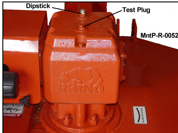
SECONDARY GEARBOX
